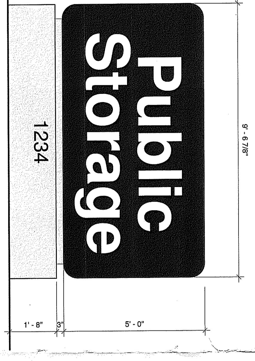
2 MONUMENT SIGN ELEVATION SK-1 SCALE: 1/2" = 1'-0"
