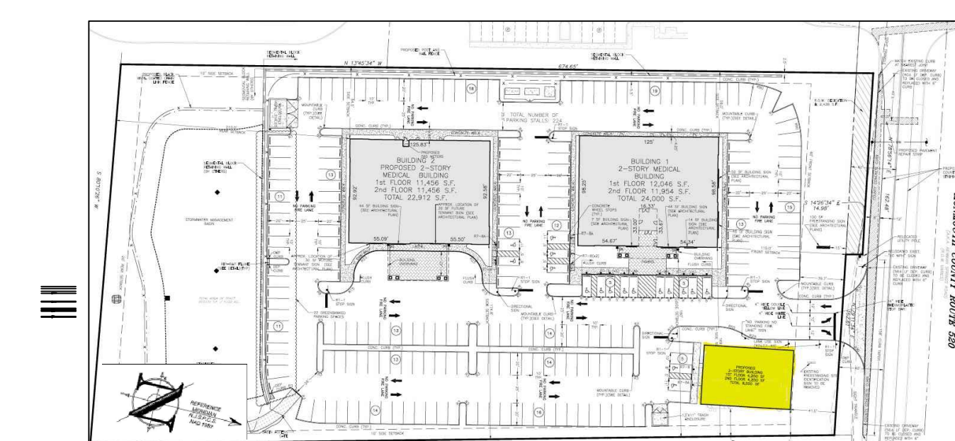
SITE PLAN
